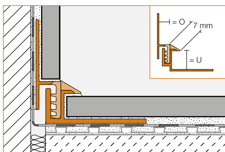
Schlüter®-DILEX-EK
